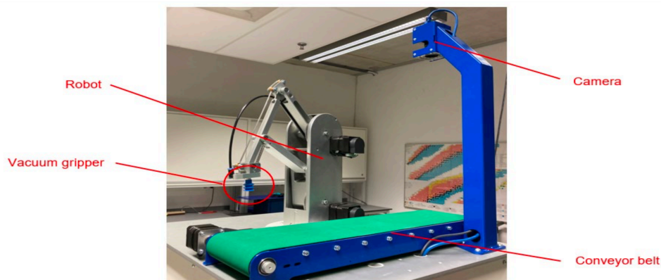
Fig. 1. Robot arm in the lab.
